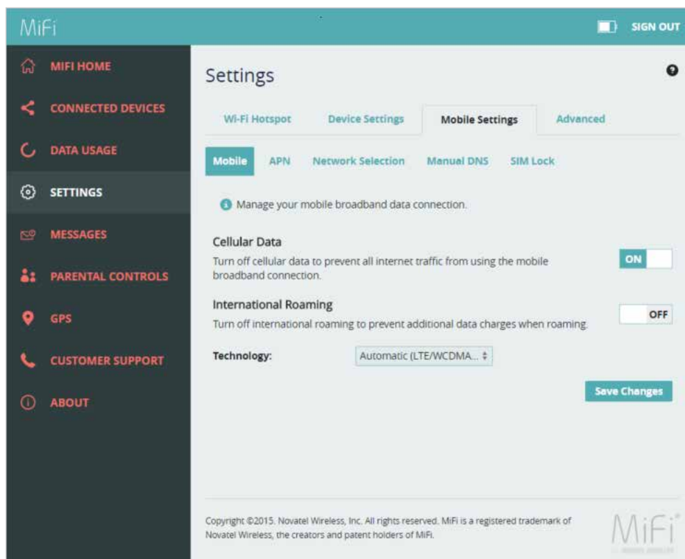
Settings - Mobile Settings
