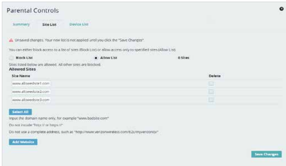
MiFi 6630 Parental Controls Site List - Allow List Add
