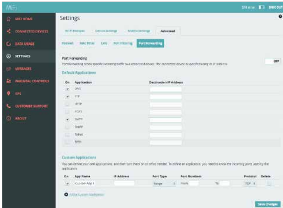
MiFi 6630 Settings Advanced - Port Forwarding
