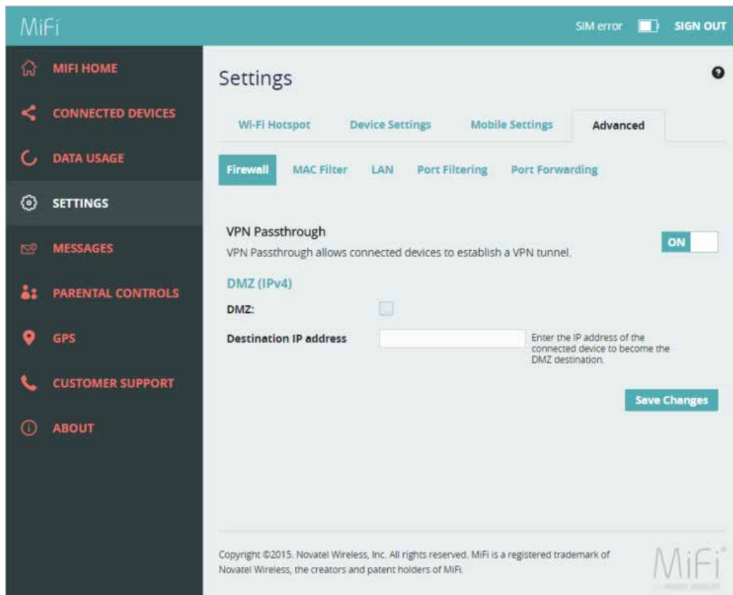
MiFi 6630 Settings Advanced - Firewall
