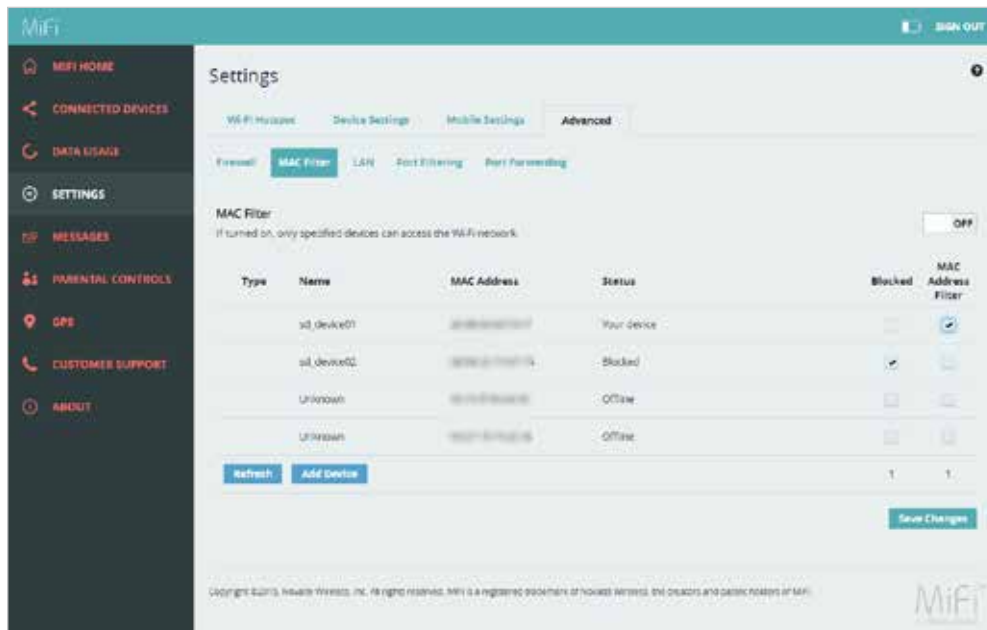
MiFi 6630 Settings Advanced - MAC Filter
