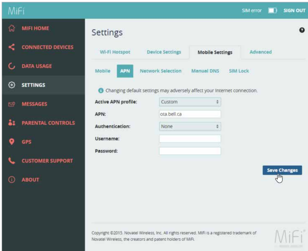
Save Custom APN Profile
