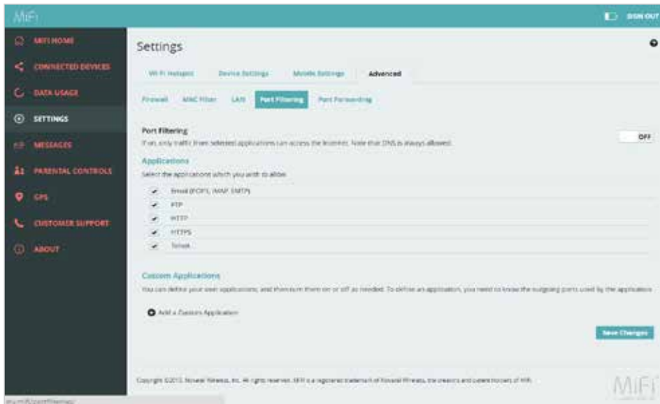
MiFi 6630 Settings Advanced - Port Filtering
